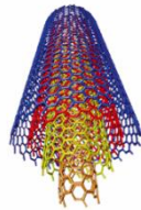
Carbon Nanotubes
